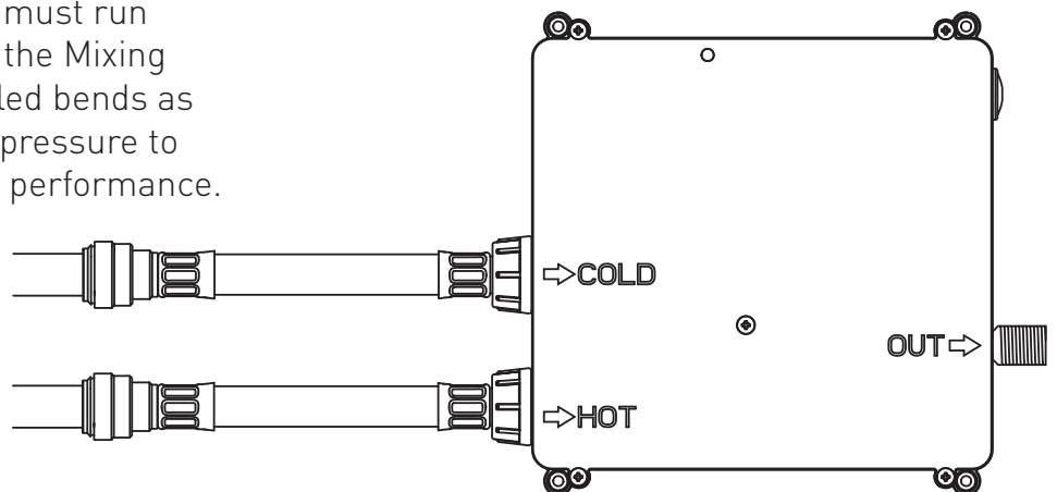
1/2" BSP Flexi Tails
