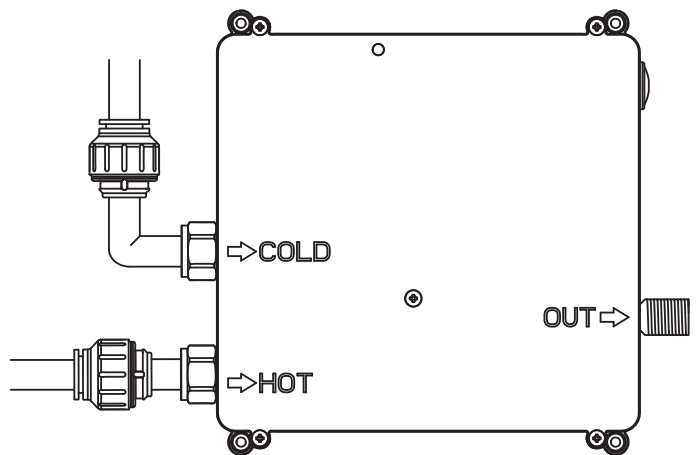
1/2" BSP Push-fit Connectors
