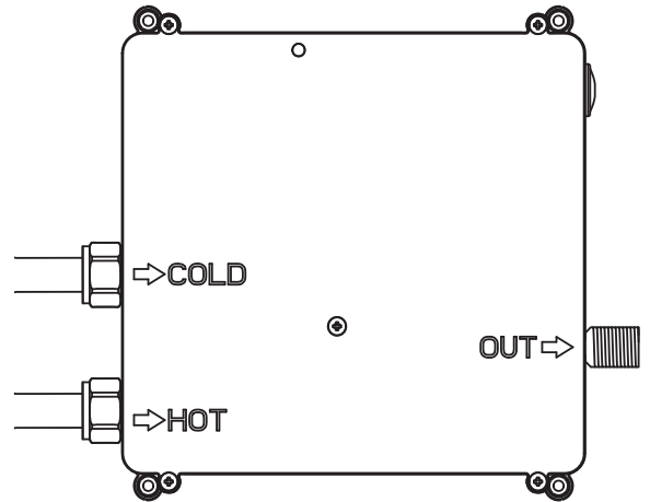
15mm Pipe work - 1/2" BSP connectors
