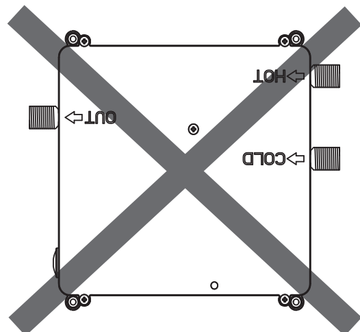
DO NOT INSTALL UPSIDE DOWN ON THE WALL!
